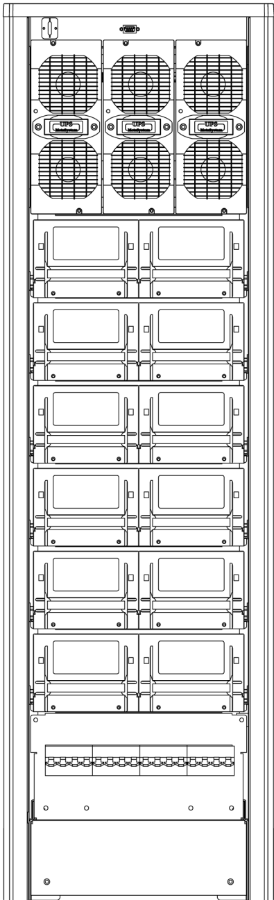
UPS Trimod® 10/15/20
