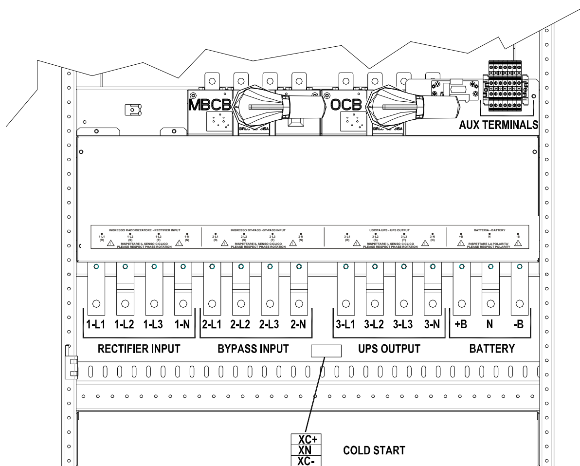
Picture 8A – Terminal board KEOR HPE 200-250 kVA
