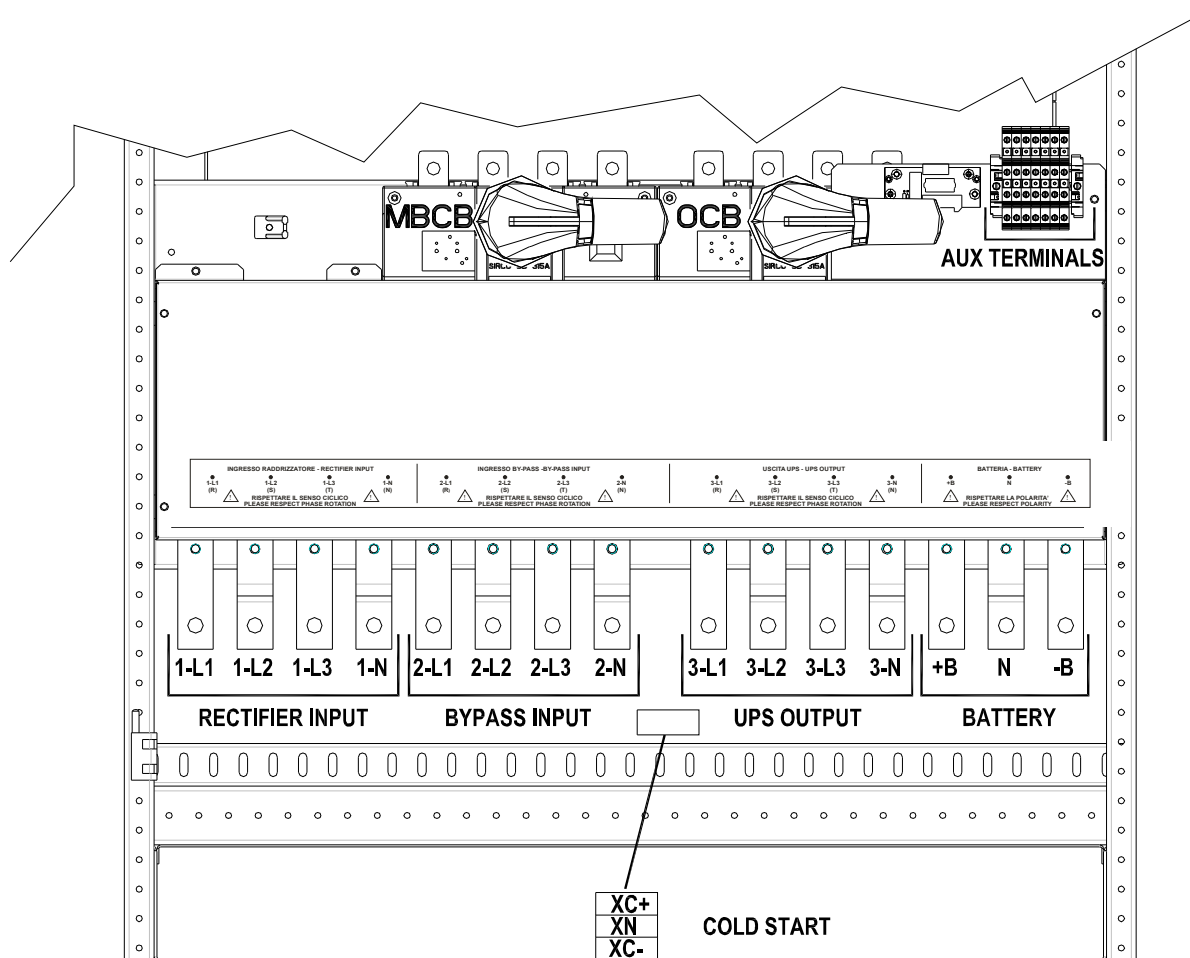
Picture 8B – Terminal board KEOR HPE 300 kVA
