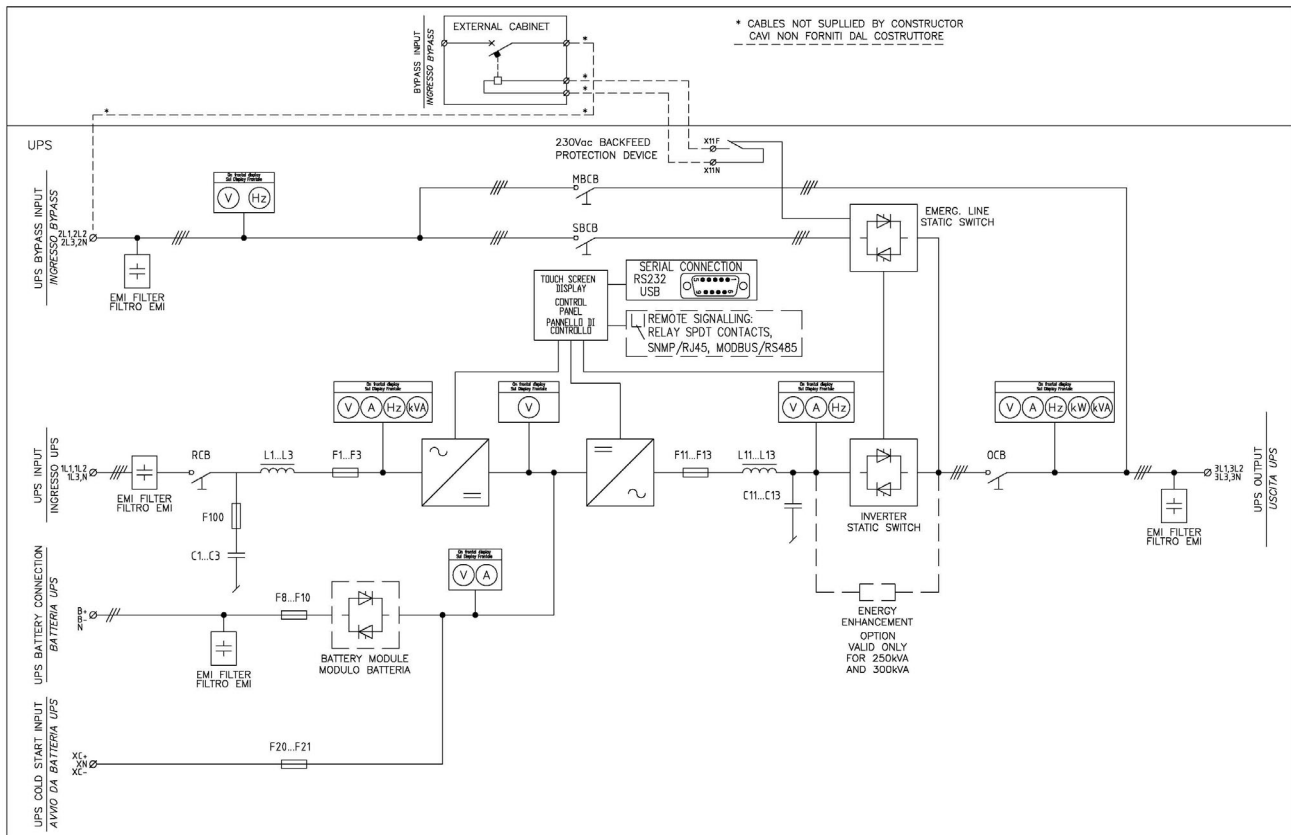
Picture 8 – Single Line Diagram KEOR HPE 200-250-300kVA with connection to external device
