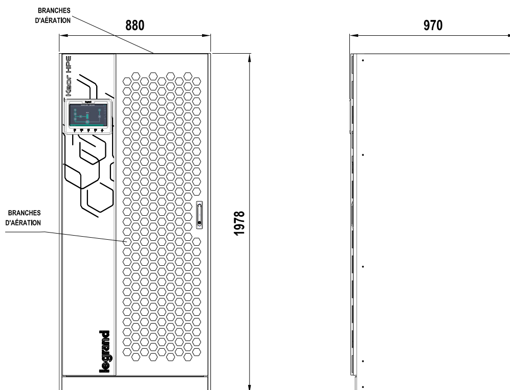
Illustration 4 – Dimensions globales
