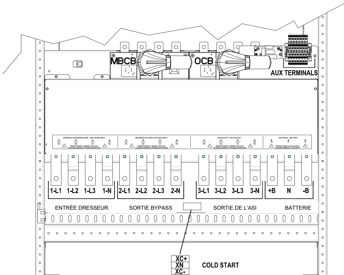
Illustration 8B – Borniers KEOR HPE 300 kVA
