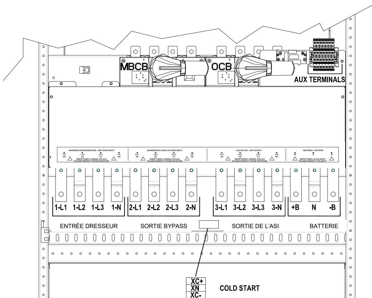
Illustration 8A – Borniers KEOR HPE 200-250 kVA
