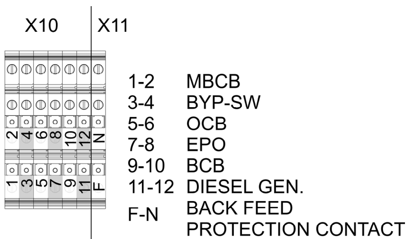
Picture 9 – Auxiliary terminals of KEOR HPE 200-250-300 kVA
