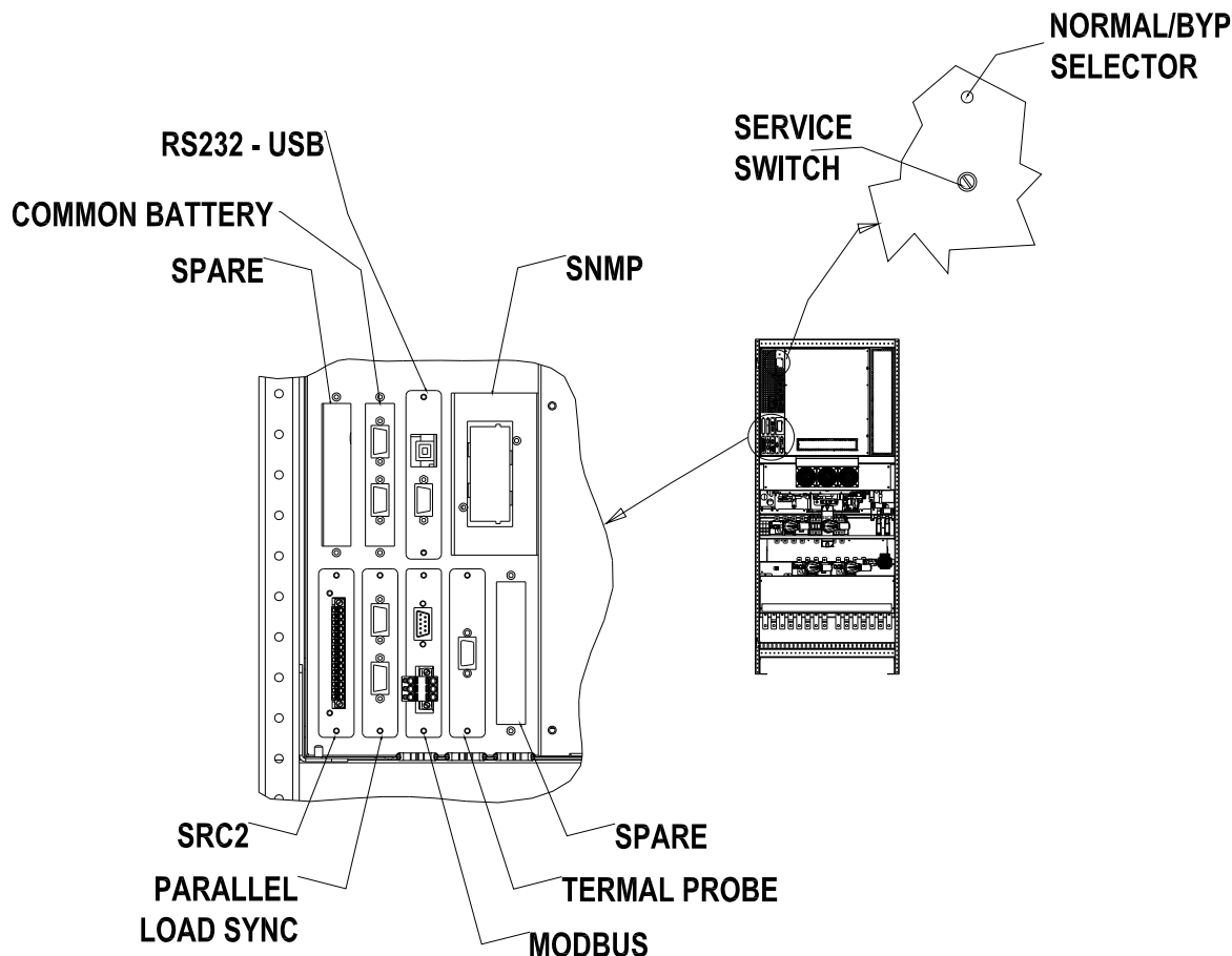
Picture 10 – Position of the serial interfaces of KEOR HPE 200-250-300 kVA
